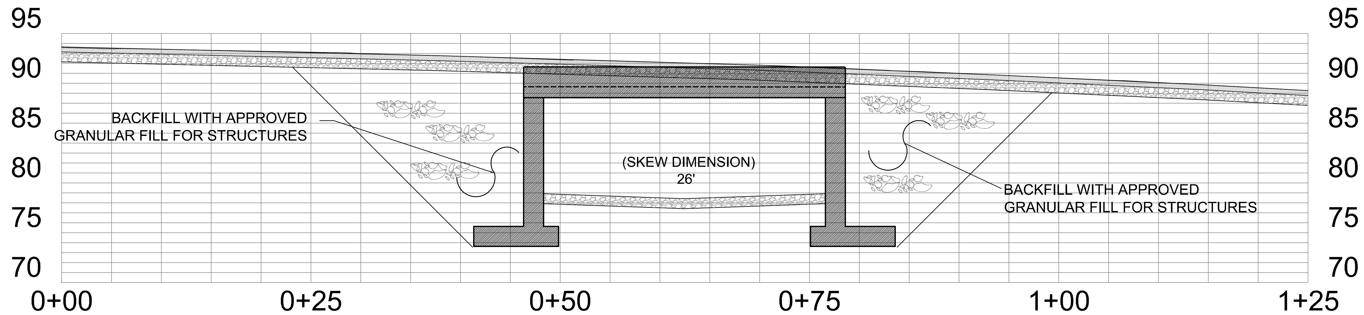
ROAD PROFILE SECTION B-B' 1"= 5'
