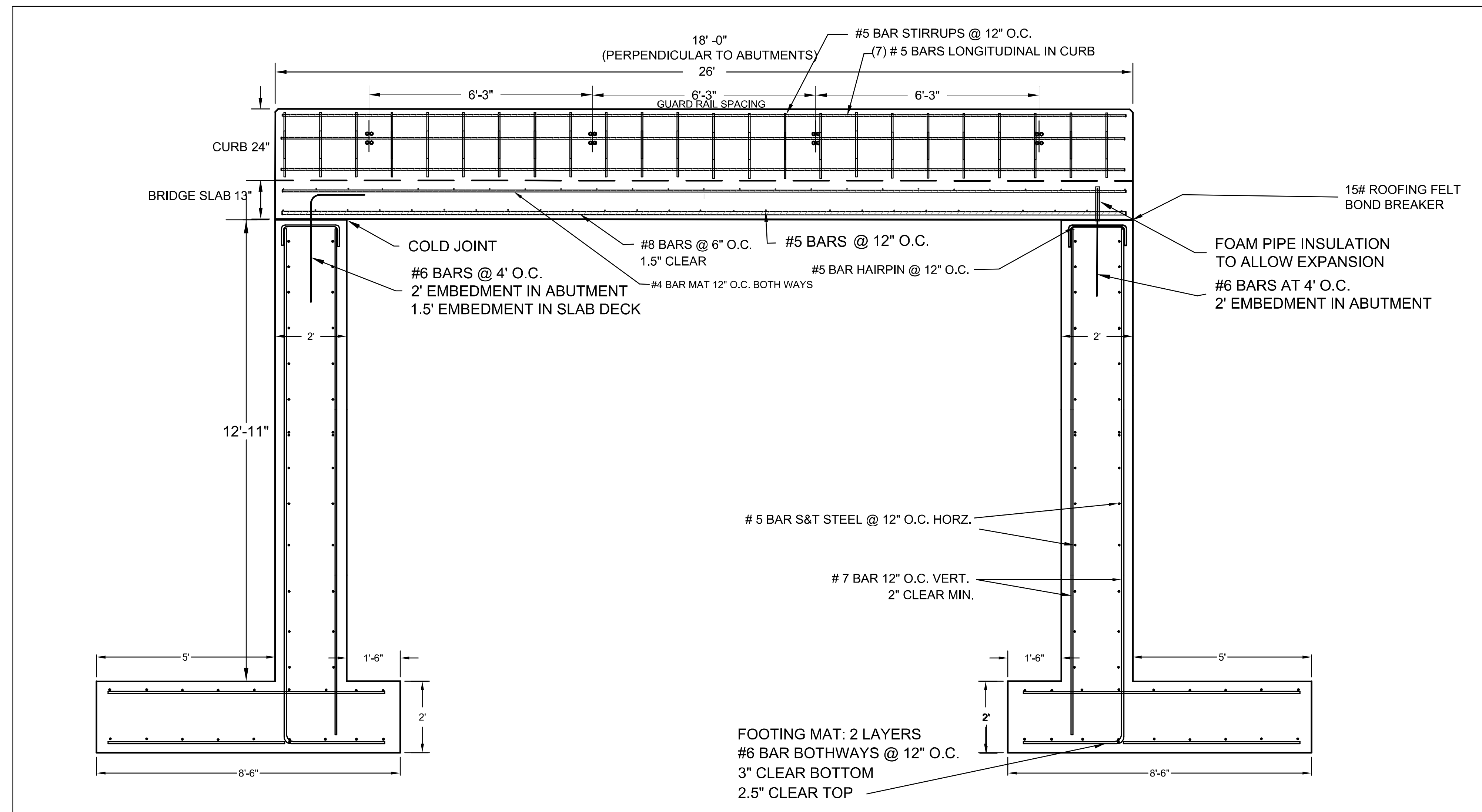
BRIDGE CROSS SECTION 1"=2' H&V
