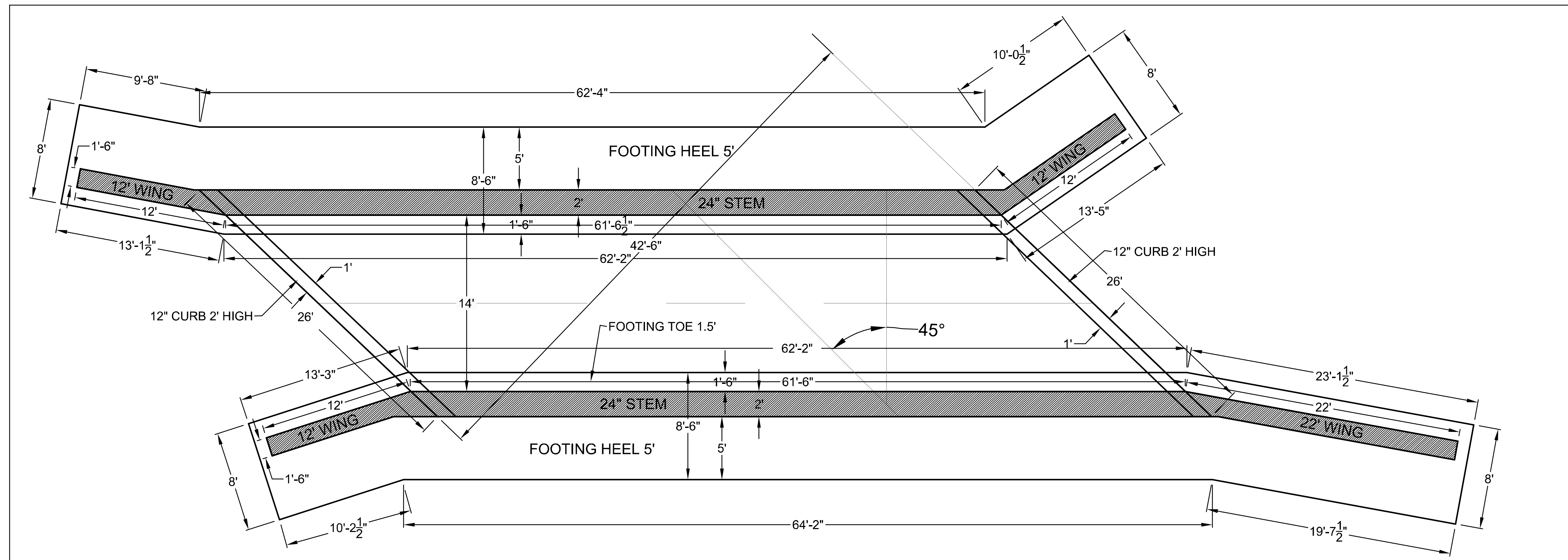
PLAN VIEW OF BRIDGE & FOOTINGS SCALE: 1"=5'
